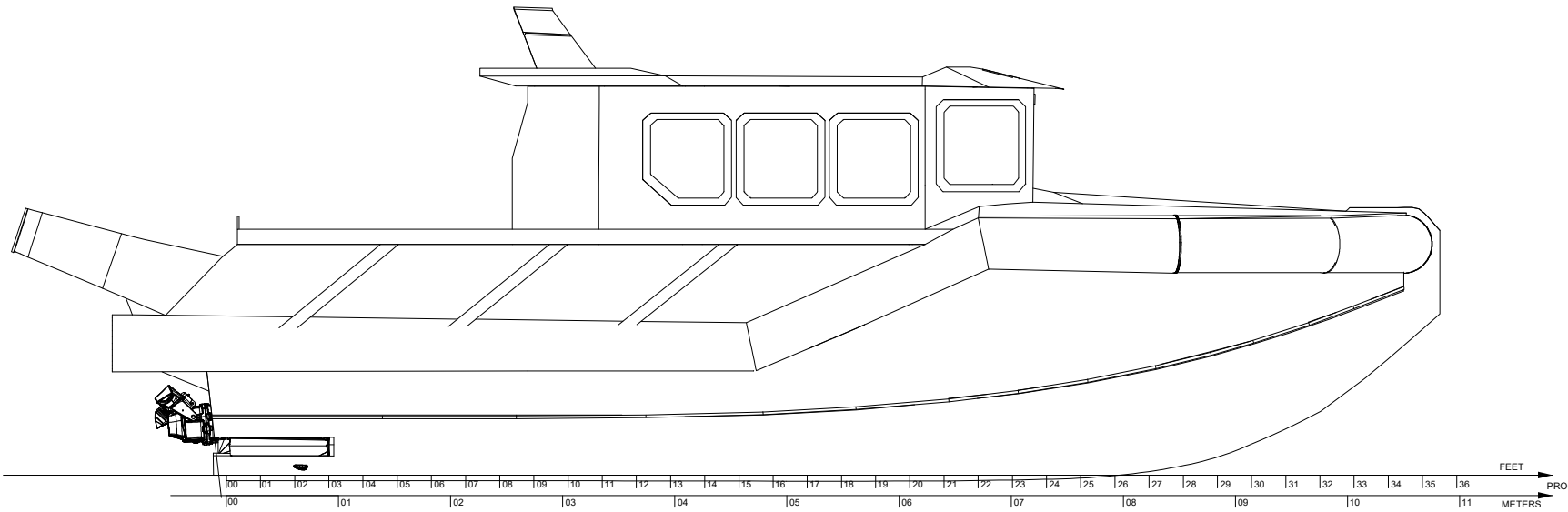
OUTBOARD PROFILE
