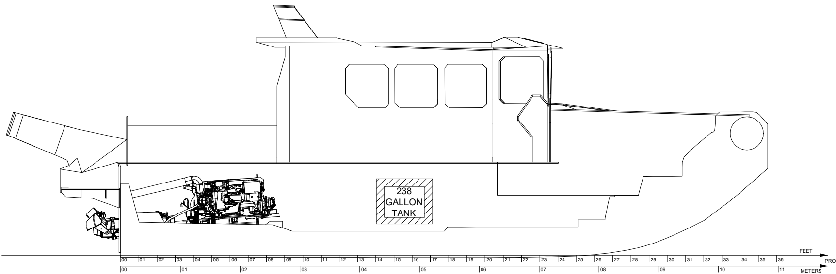
INBOARD PROFILE
