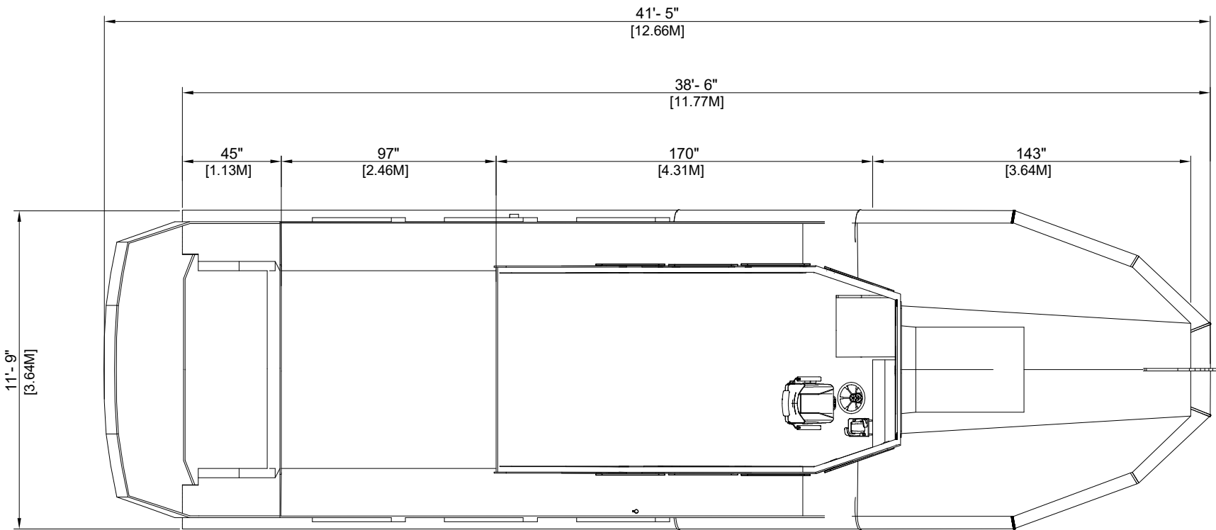
INBOARD PLAN VIEW
