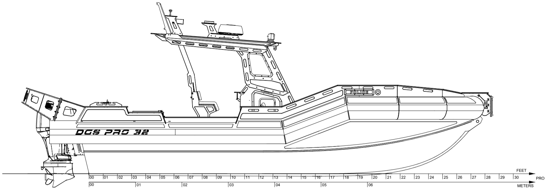
OUTBOARD PROFILE
