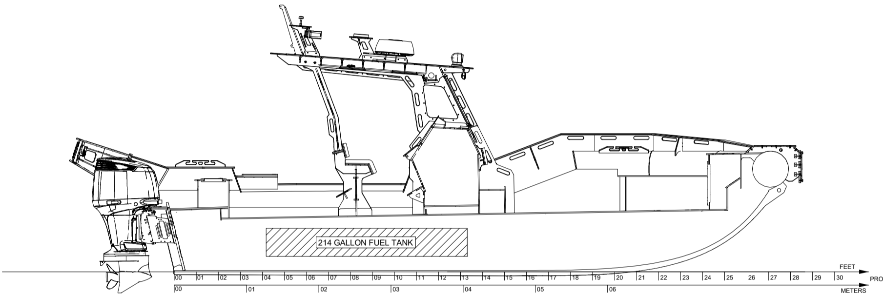
INBOARD PROFILE
