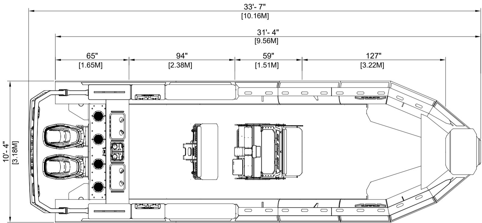
INBOARD PLAN VIEW
