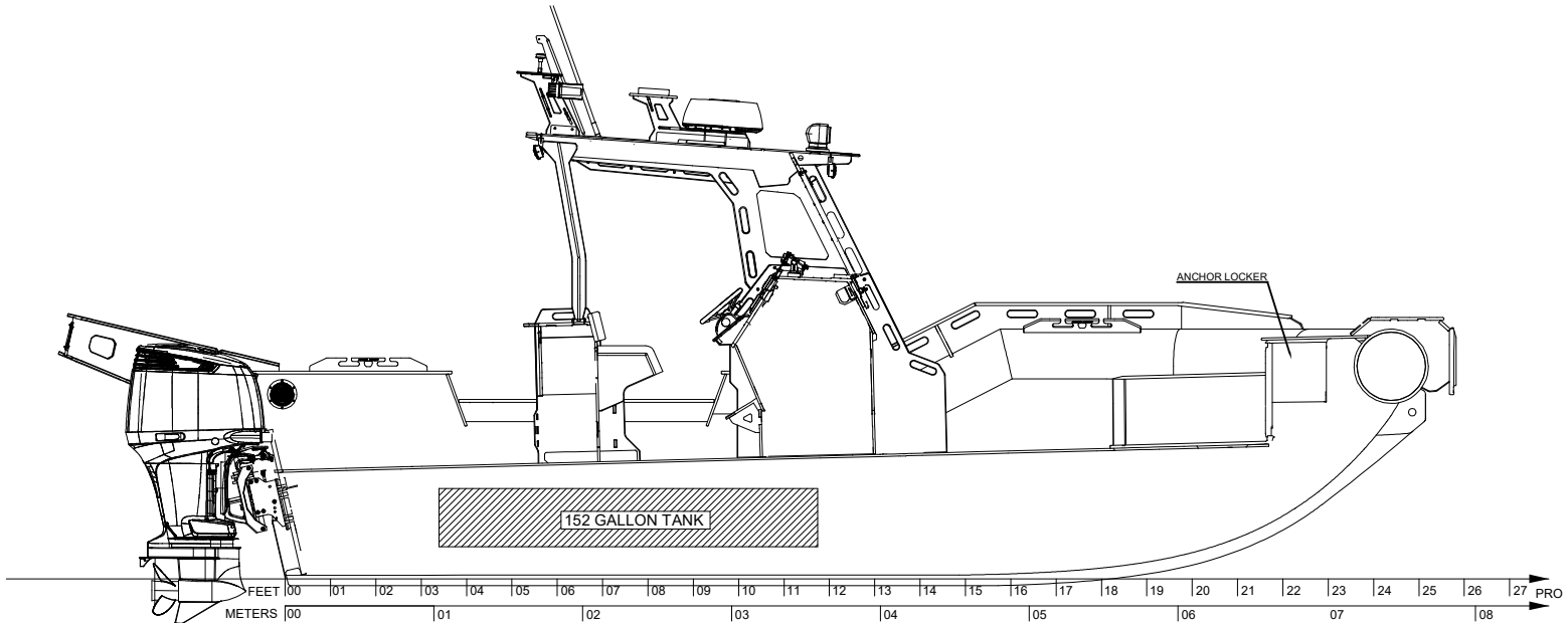
INBOARD PROFILE
