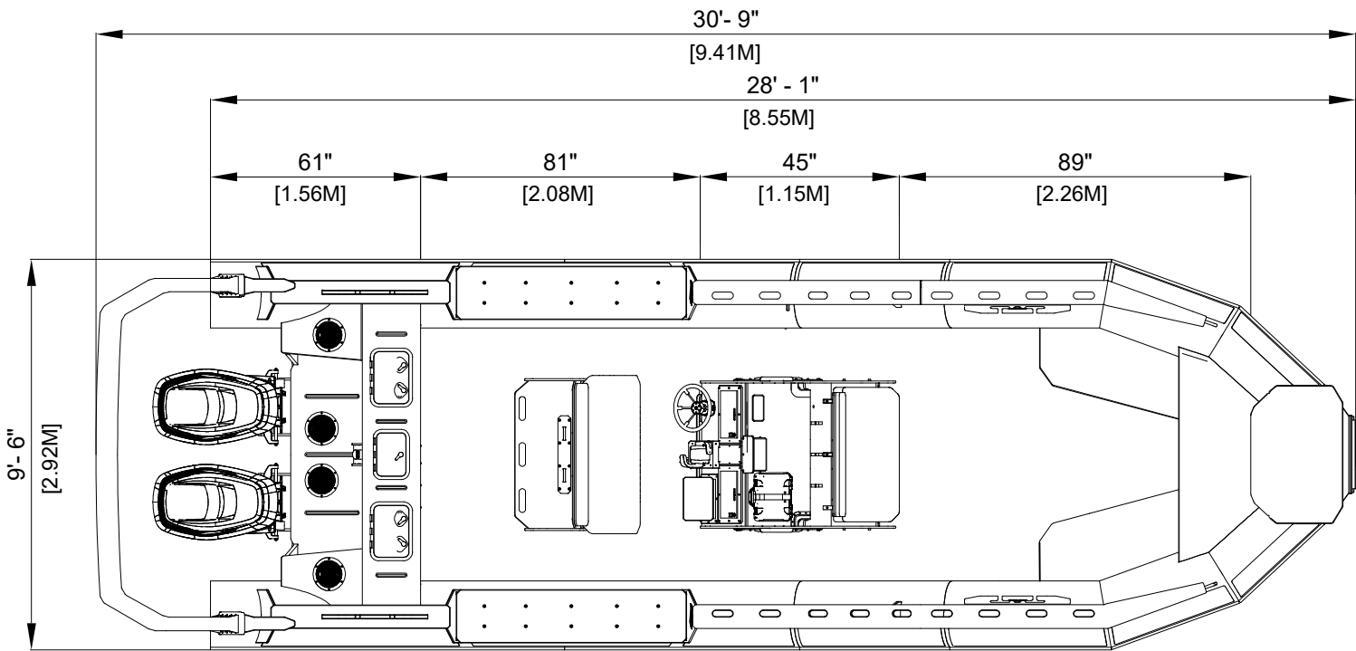
INBOARD PLAN VIEW
