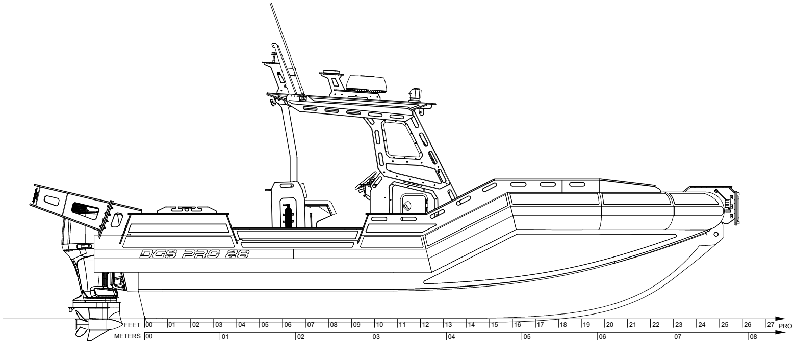
OUTBOARD PROFILE
