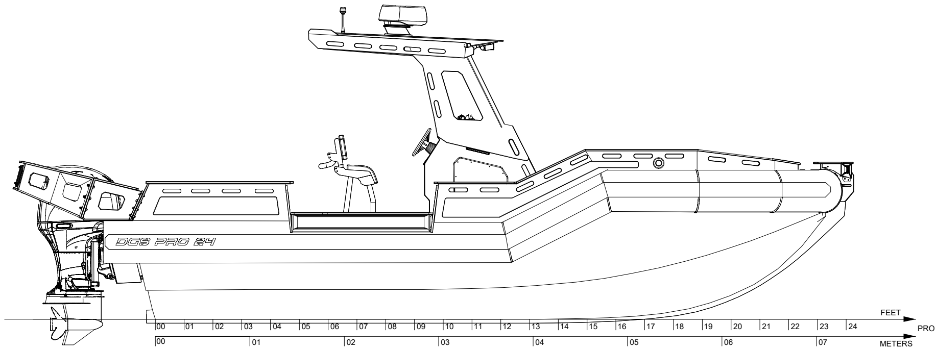
OUTBOARD PROFILE
