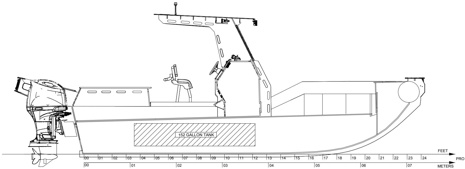
INBOARD PROFILE
