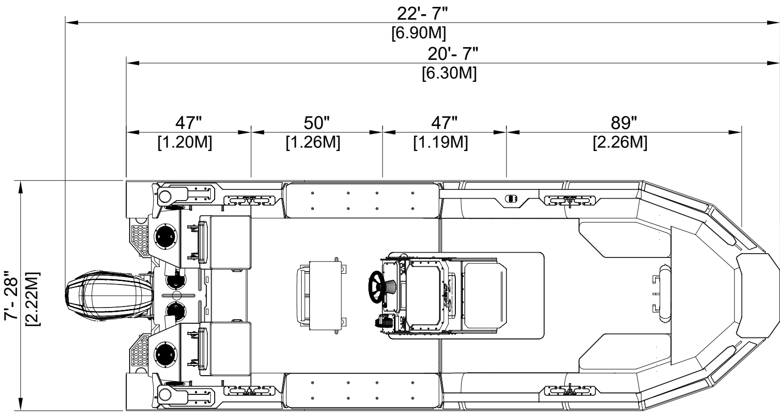
INBOARD PLAN VIEW
