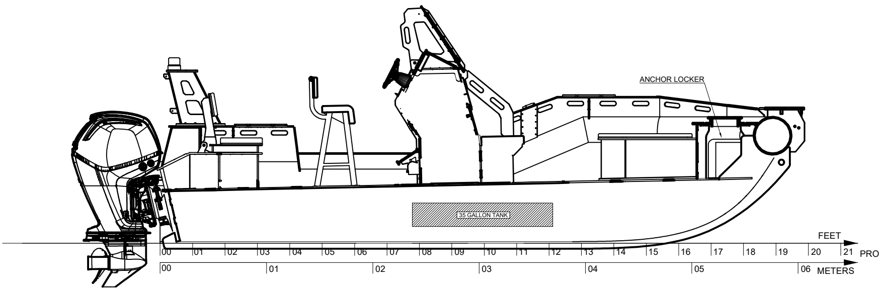
INBOARD PROFILE
