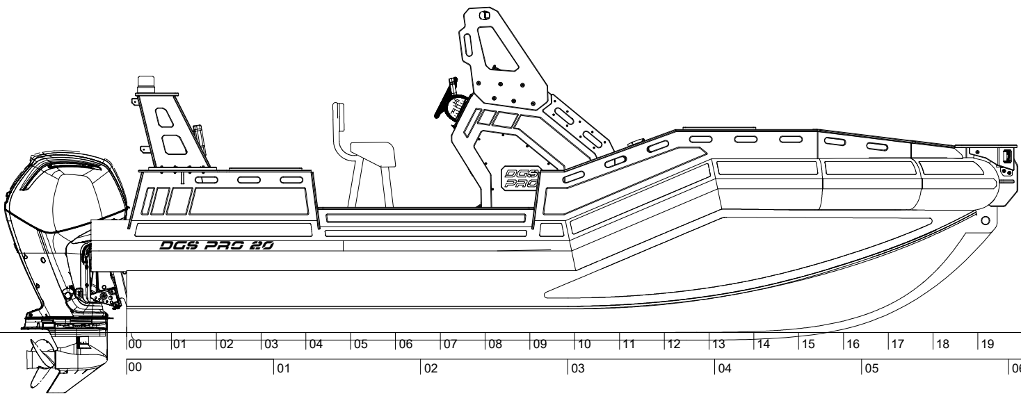
OUTBOARD PROFILE
