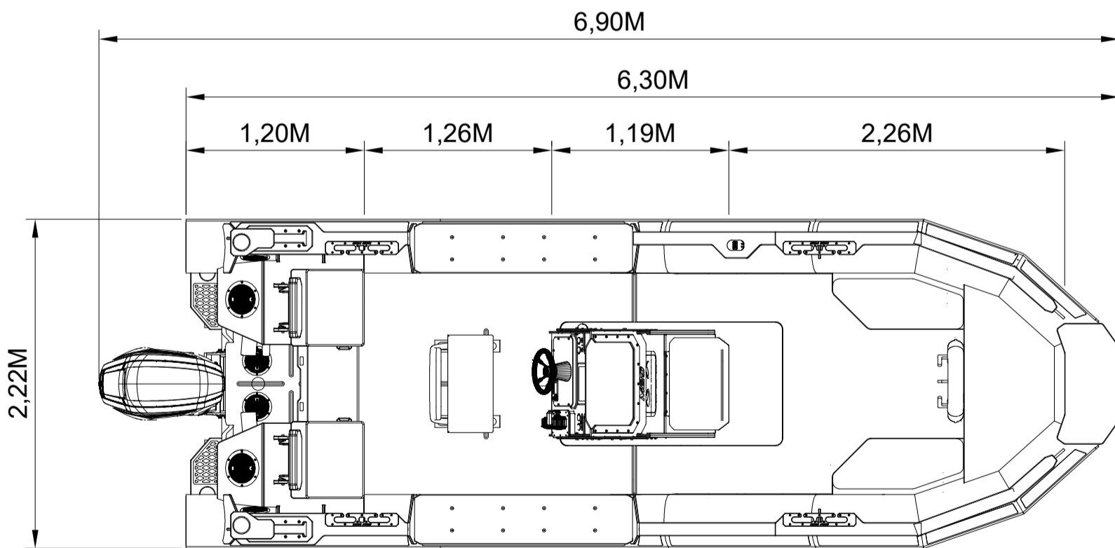
VISTA DE CONVÉS PRINCIPAL
